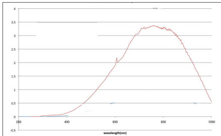
CDS-30x0 Sensitivity
