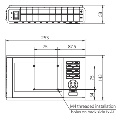
Data processor dimensions (Units : mm)
