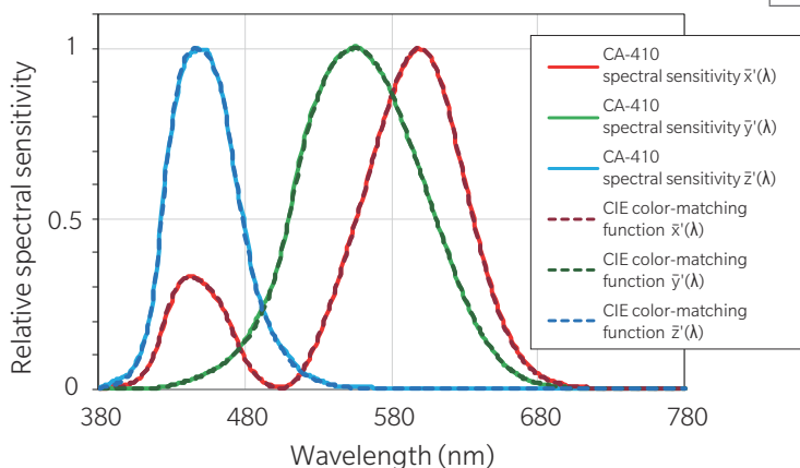
CA-410 spectral sensitivity vs. CIE 1931 color-matching functions
