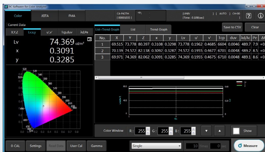
Chromaticity measurement
