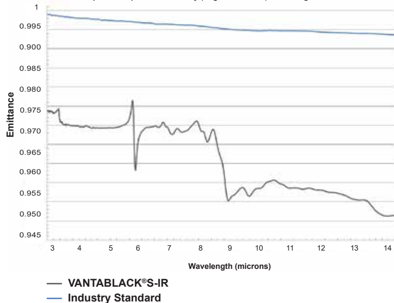
Extended Area Blackbody Surface Treatments Comparison Hemispherical Spectral Emissivity (Avg Polarization) at 20° Angle of Incidence
