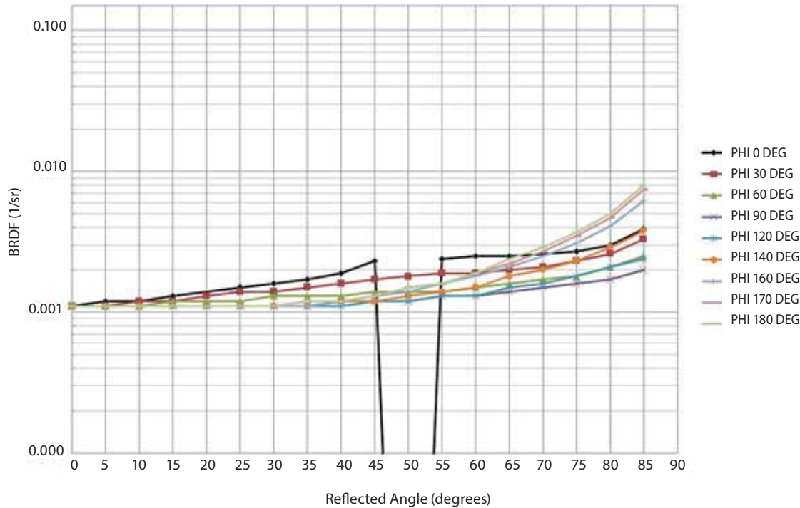
MWIR BRDF at 50 DEGREE ANGLE OF INCIDENCE VANTABLACK®S-IR has significantly better absorption and labertian reflectance at high angles of incidence and off specular compared to paint
