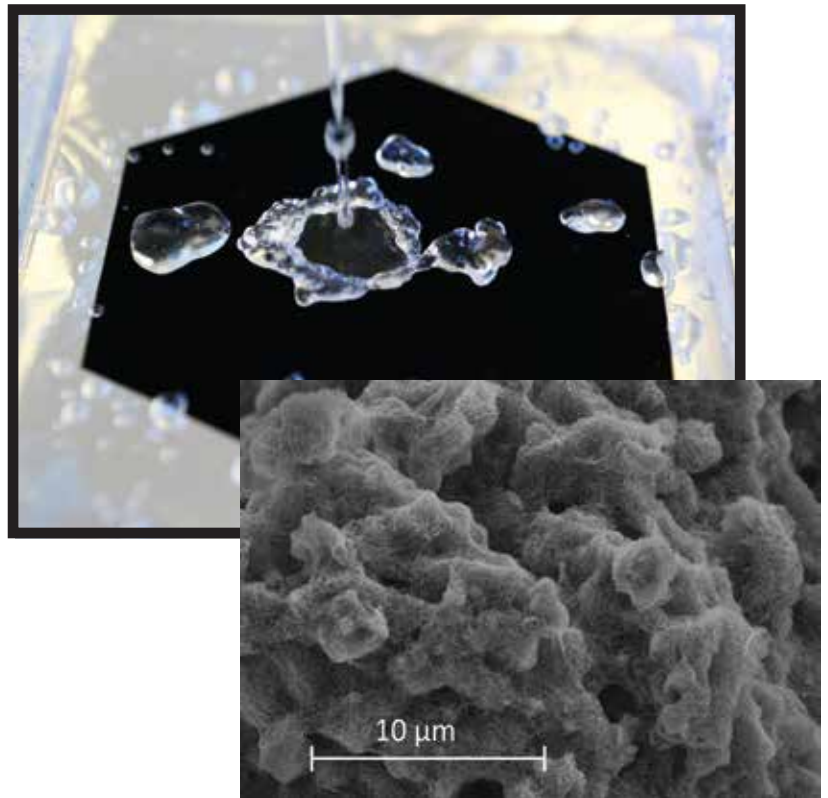
VANTABLACK®S-IR scanning electron microscope (SEM)
