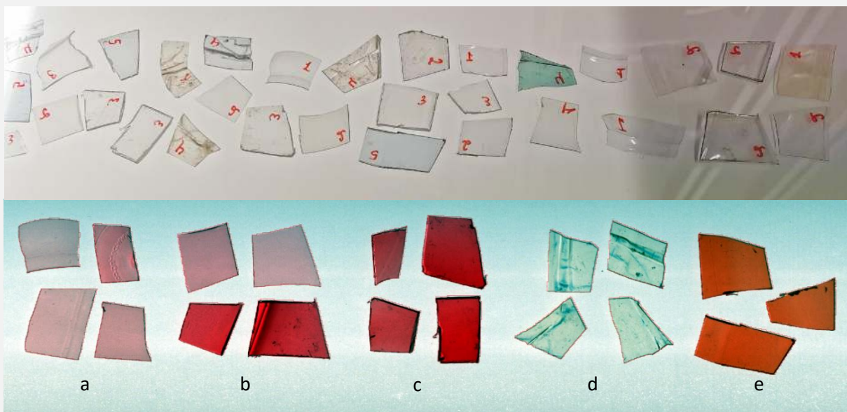
A normal RGB image of the mixed plastic waste (top) and a SWIR-based false colour image (bottom) of five types of plastic waste: PET Bottle (a), PET Sheet (b), PET G (c), PVC (d) and PC (e). The samples appear transparent in the visual range are difficult to identify accurately and repeatably by visual inspection.
