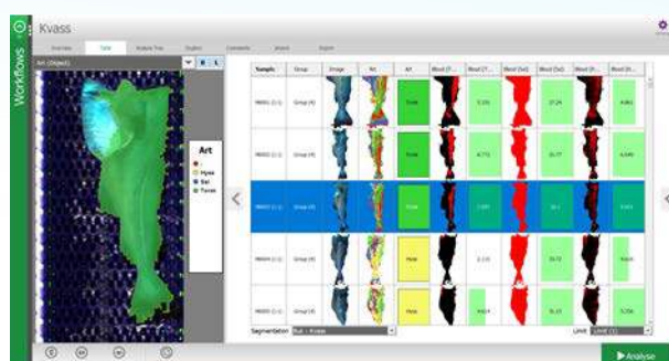
Real-time classification
