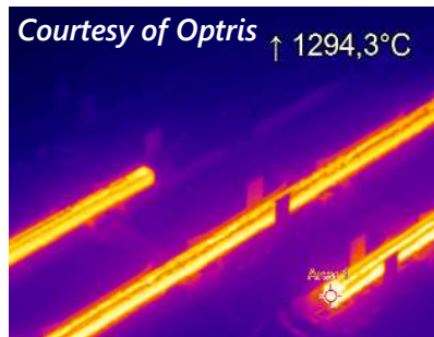
Thermographic image of steel slabs captured with PIIM
