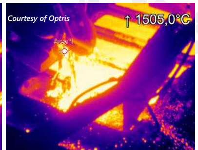
Non-contact measurement of casting temperature with PIIM
